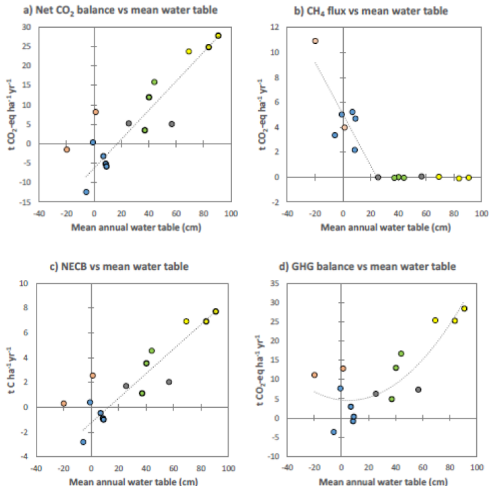
Figure 1: Observed relationships between a) net CO 2 flux; b) terrestrial CH 4 flux, c) Net Ecosystem Carbon Balance and d) overall GHG balance (excluding N 2 O) and mean measured water-table depth for all study sites. Sites are colour-coded as: blue = conservation-managed fen; orange = re-wetted raised bog; grey = extraction site; green = grassland; yellow = arable.
