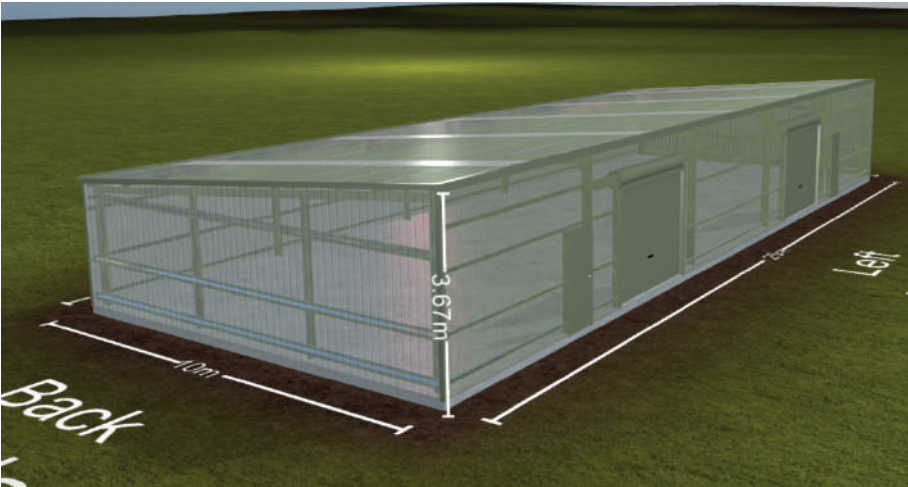
FRONT ASPECT VIEWED FROM SOUTH WEST - TRANSPARENT FRAME
