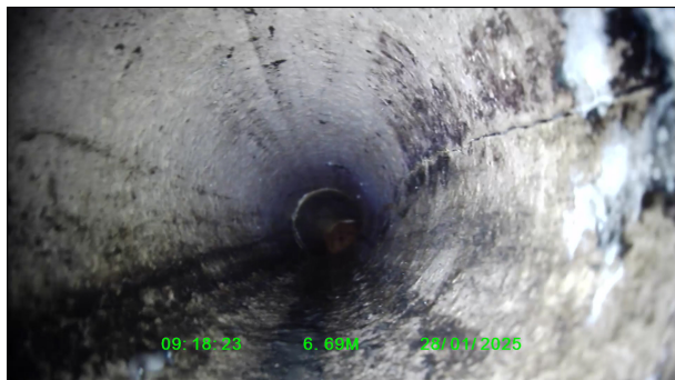
Photo: 1_1_17_A.jpg 6.7m, Fracture, longitudinal at joint, at 3 o'clock, Start
