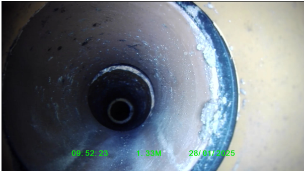
Photo: 4_4_42_A.jpg 1.4m, Open joint, medium Remarks: joint pulled
