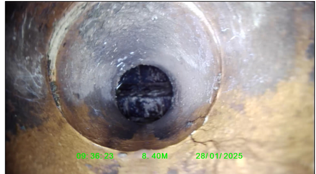
Photo: 3_3_33_A.jpg 8.5m, Roots, fine at joint
