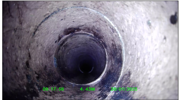
Photo: 1_1_14_A.jpg 4.5m, Fracture, circumferential, from 12 to 12 o'clock
