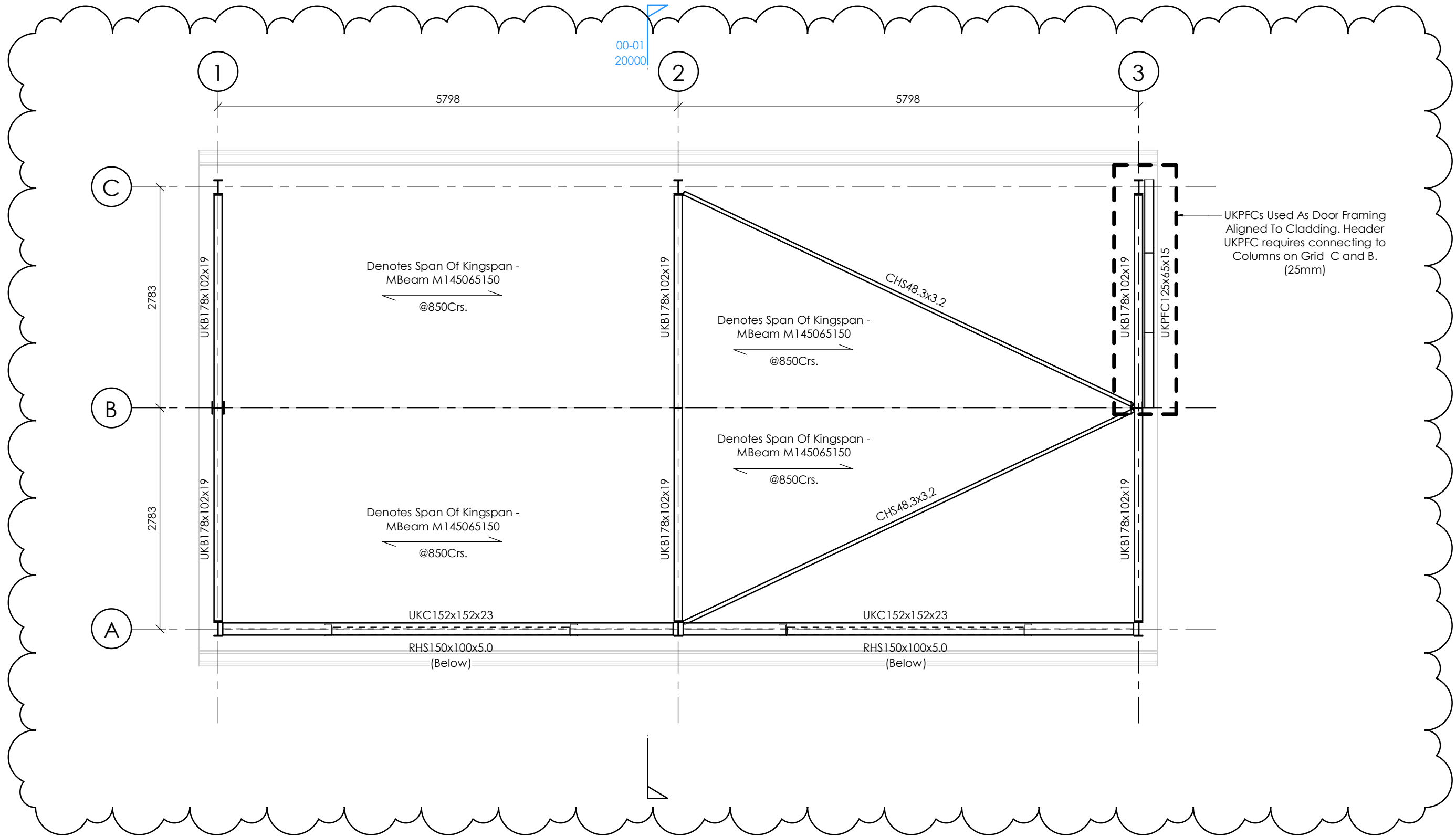
ROOF STRUCTURE LAYOUT 1 : 50
