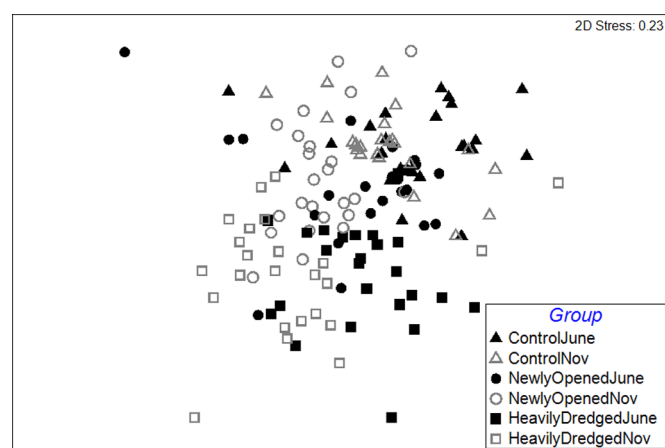
Fig. 4. Two-dimensional MDS plot derived from the log ( x+1 ) transformed similarity matrix indicating the similarity between the macrofaunal assemblages at sampling locations in June (black) and November (grey) 2015. Circles = newly dredged site/medium dredging intensity (open July–October), squares = heavily dredged site, triangles = control site.
