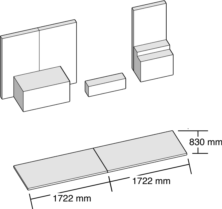
Base plinth panels. 2 @ 1722w x 830d x 40h mm
