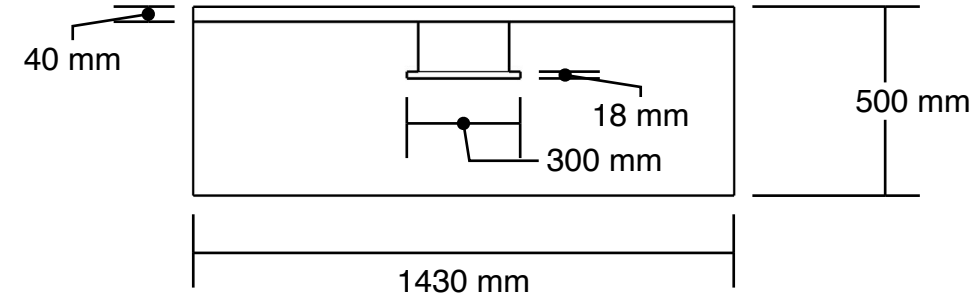
Plan 1:20 @ A3
