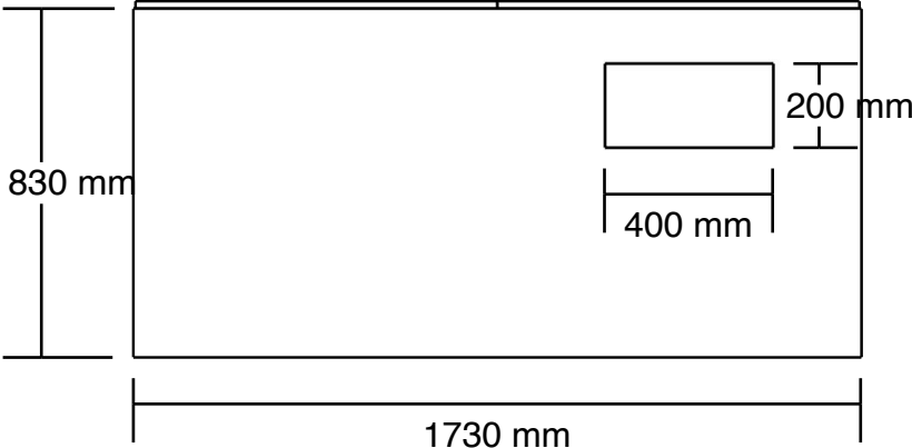
Plan 1:20 @ A3
