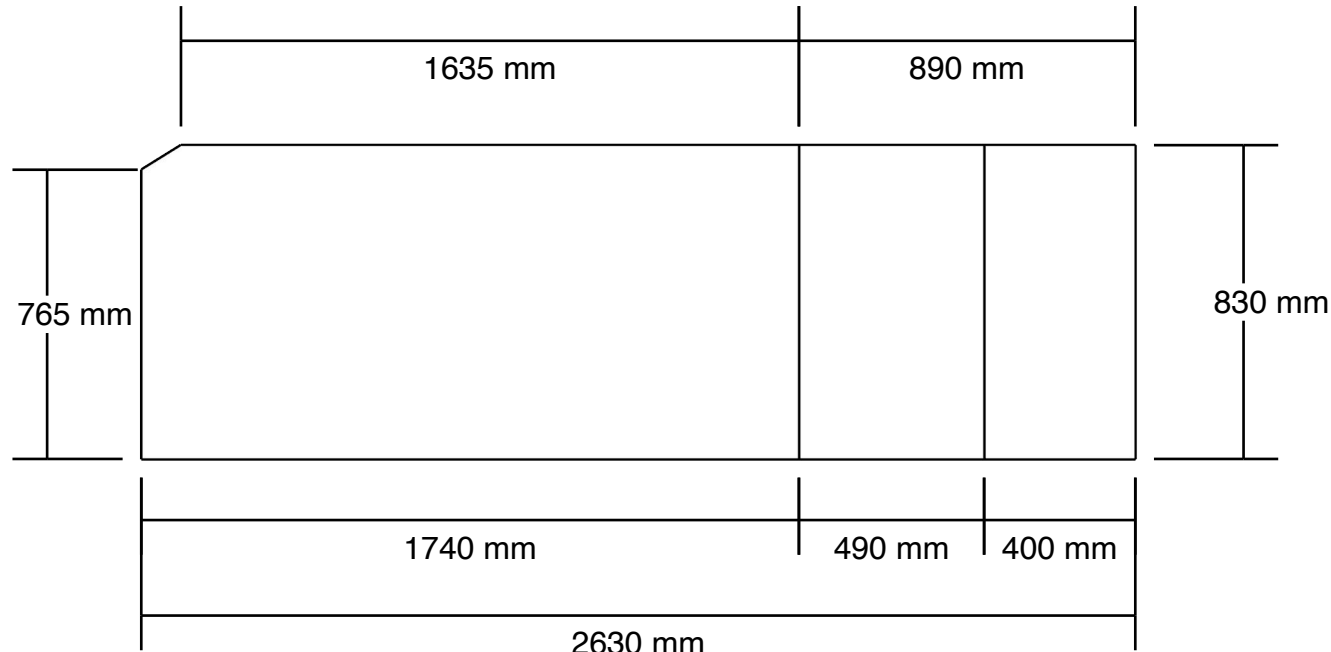
Plan 1:20 @ A3
