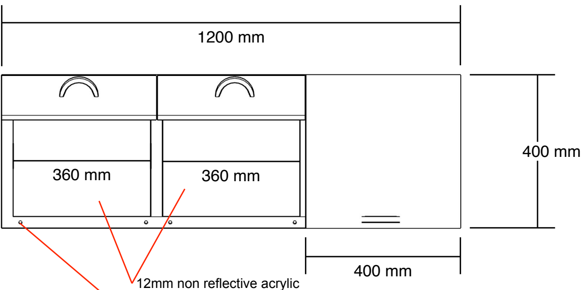
Plan 1:10 @ A3
