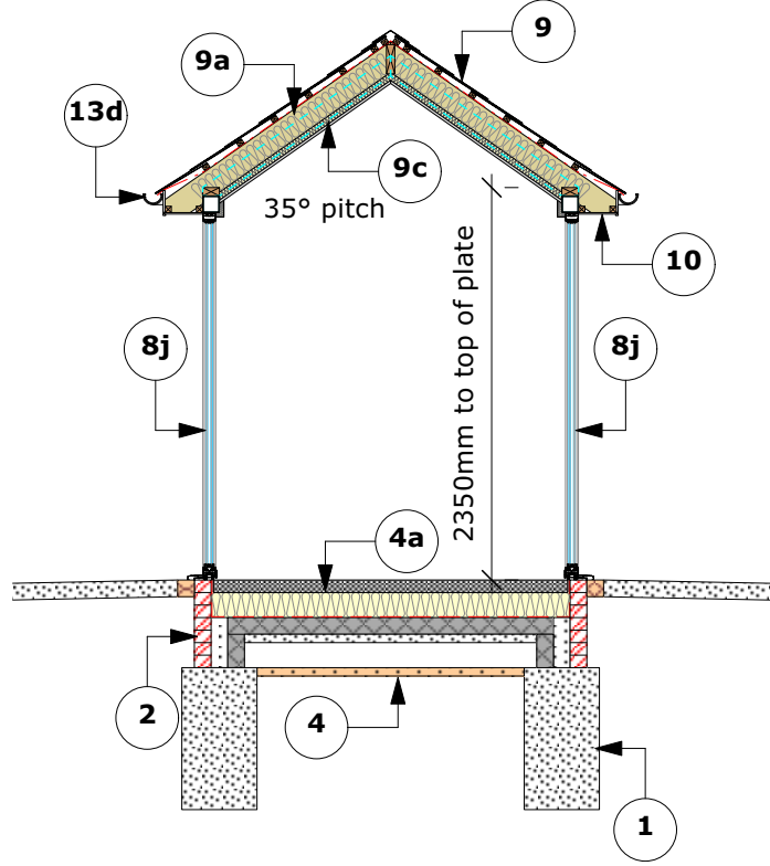
SECTION EE
