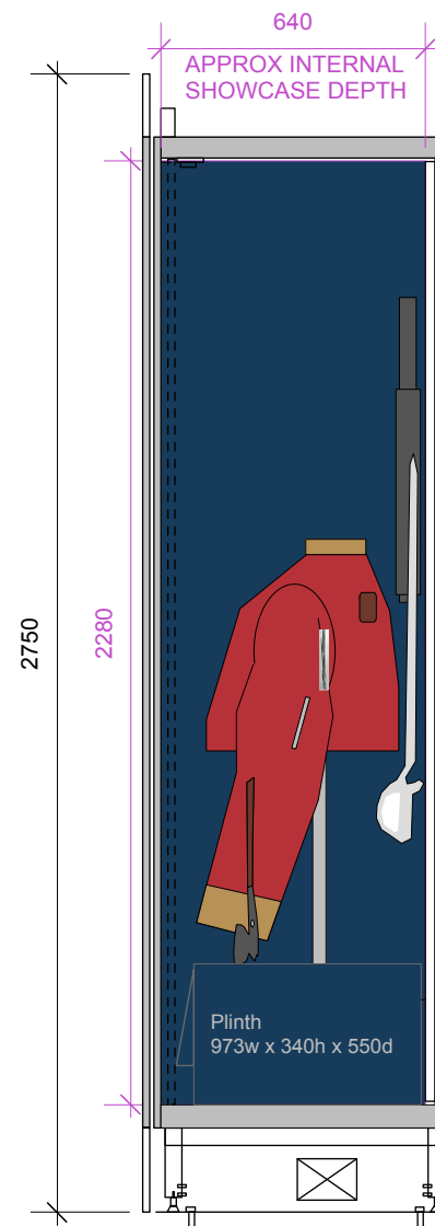
SIDE ELEVATION
