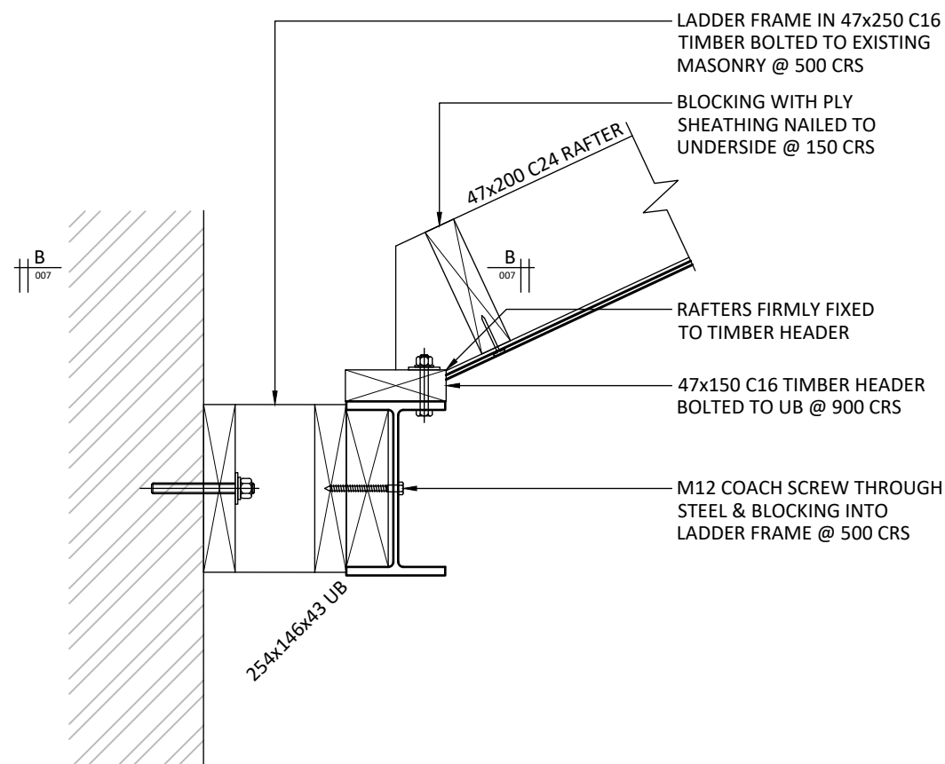
SECTION 8-8 (1:10)
