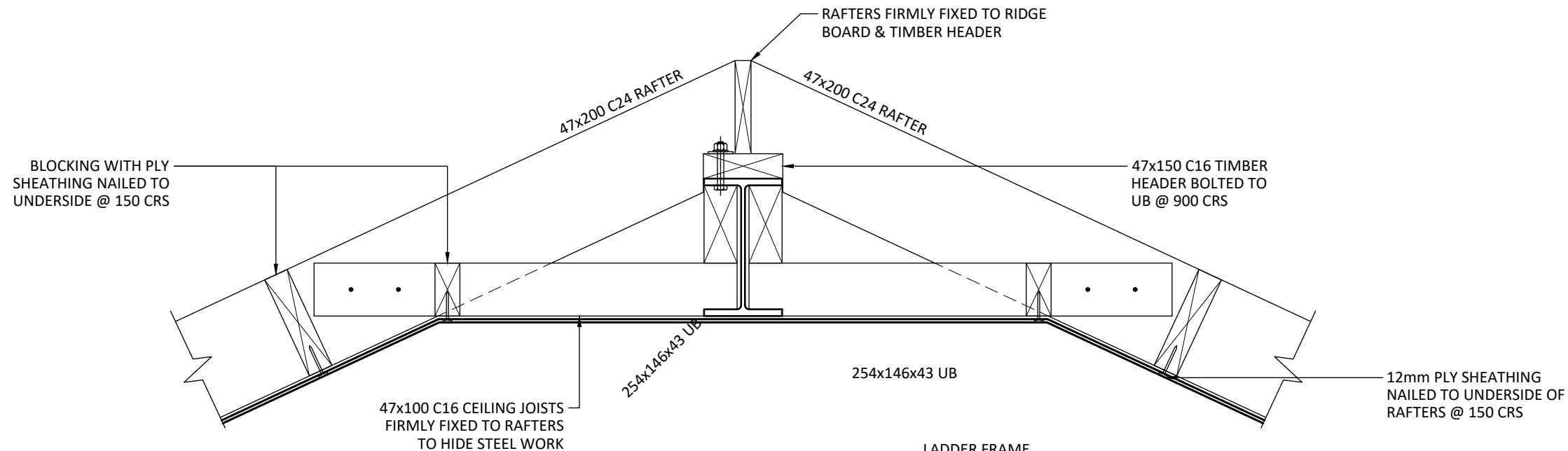
SECTION 7-7 (1:10)
