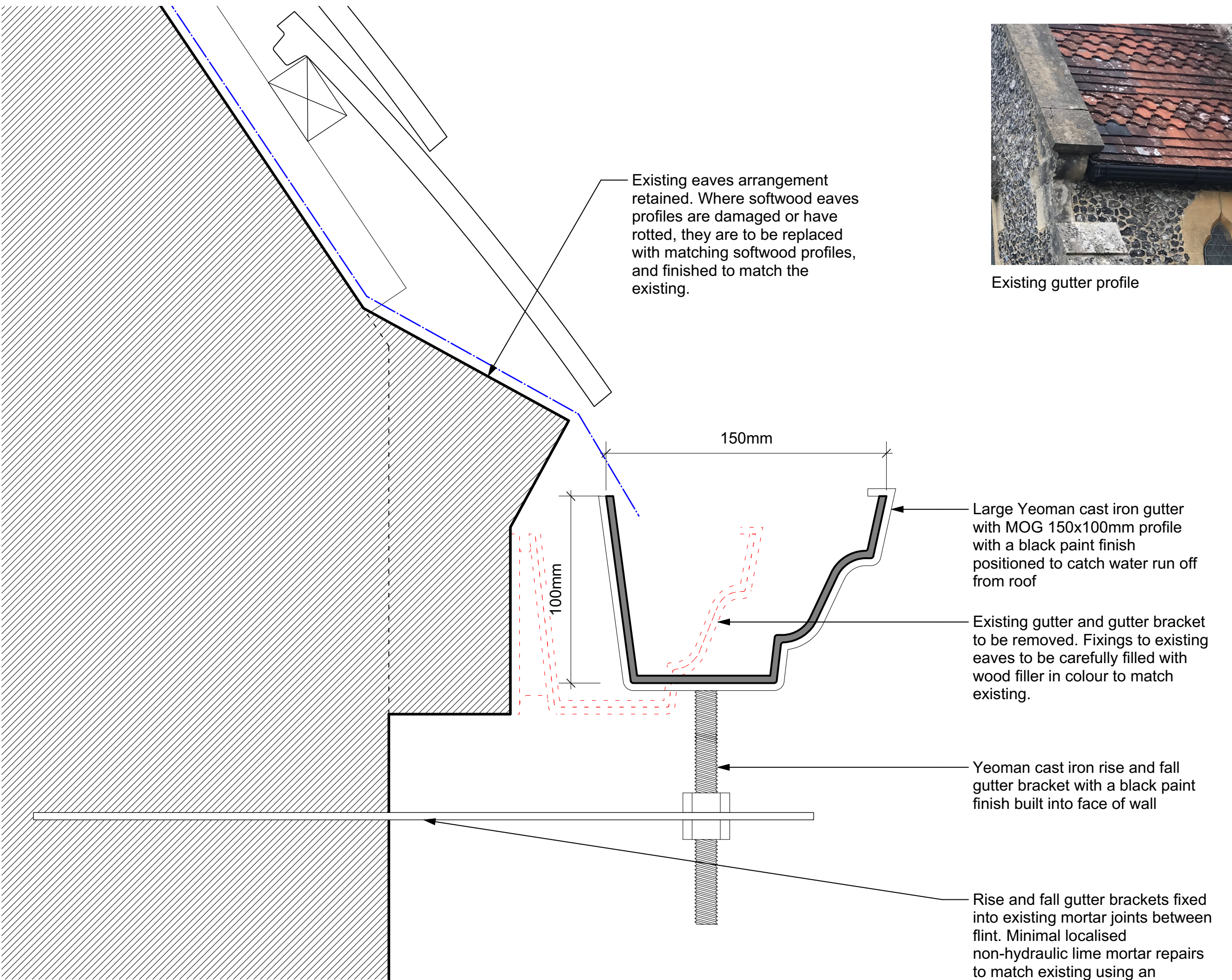
Gutter Detail 1:2 @ A3
