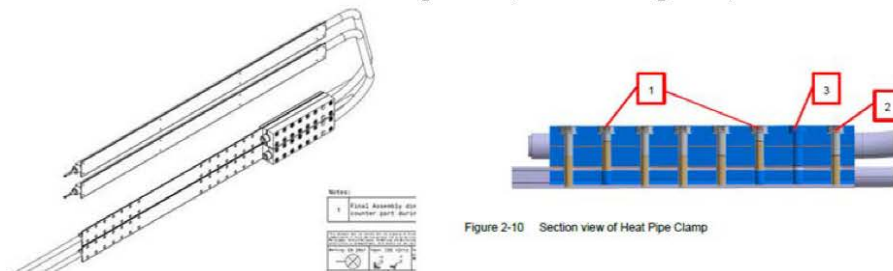
Figure 10: Foreseen Interface for RAL HPC MGSE
