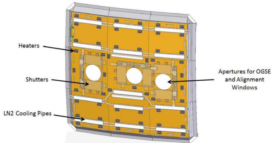
Figure 7: S5 OGSE Room Door Shroud Design
