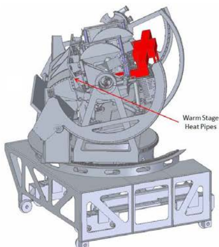
Figure 9: Warm Stage Heat Pipe
