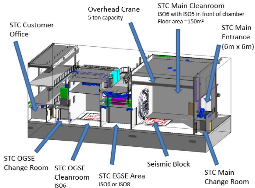
Figure 2: Section through STC Test Suite indicating key features
