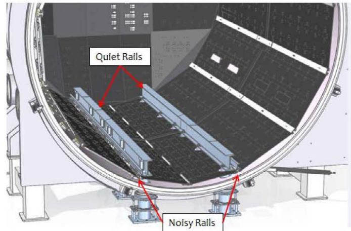
Figure 3: TVAC Chamber Quiet and Noisy Rails
