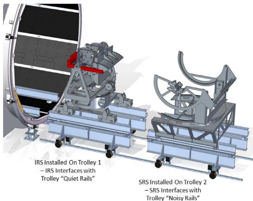
Figure 5: S5 IRS and SRS Installed on Cleanroom Trolleys
