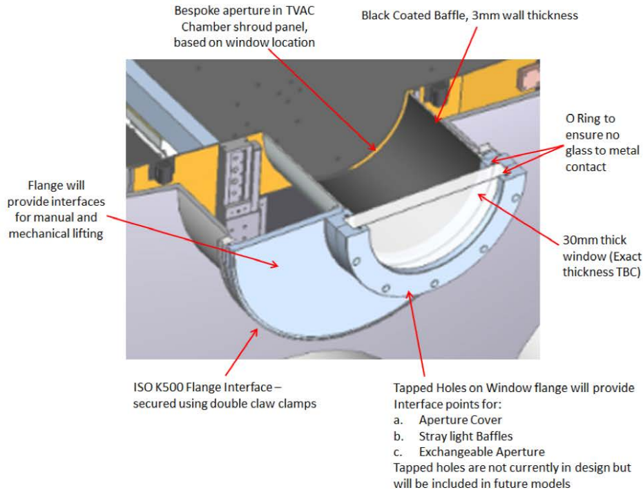
Figure 6: overview of the window flange design
