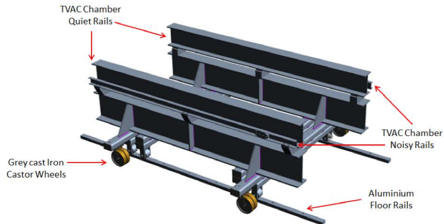
Figure 4: Cleanroom Trolley
