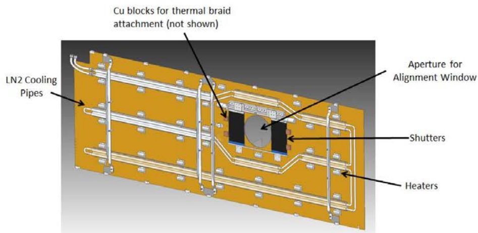
Figure 8: Service Area Alignment Window Shroud Panel Design
