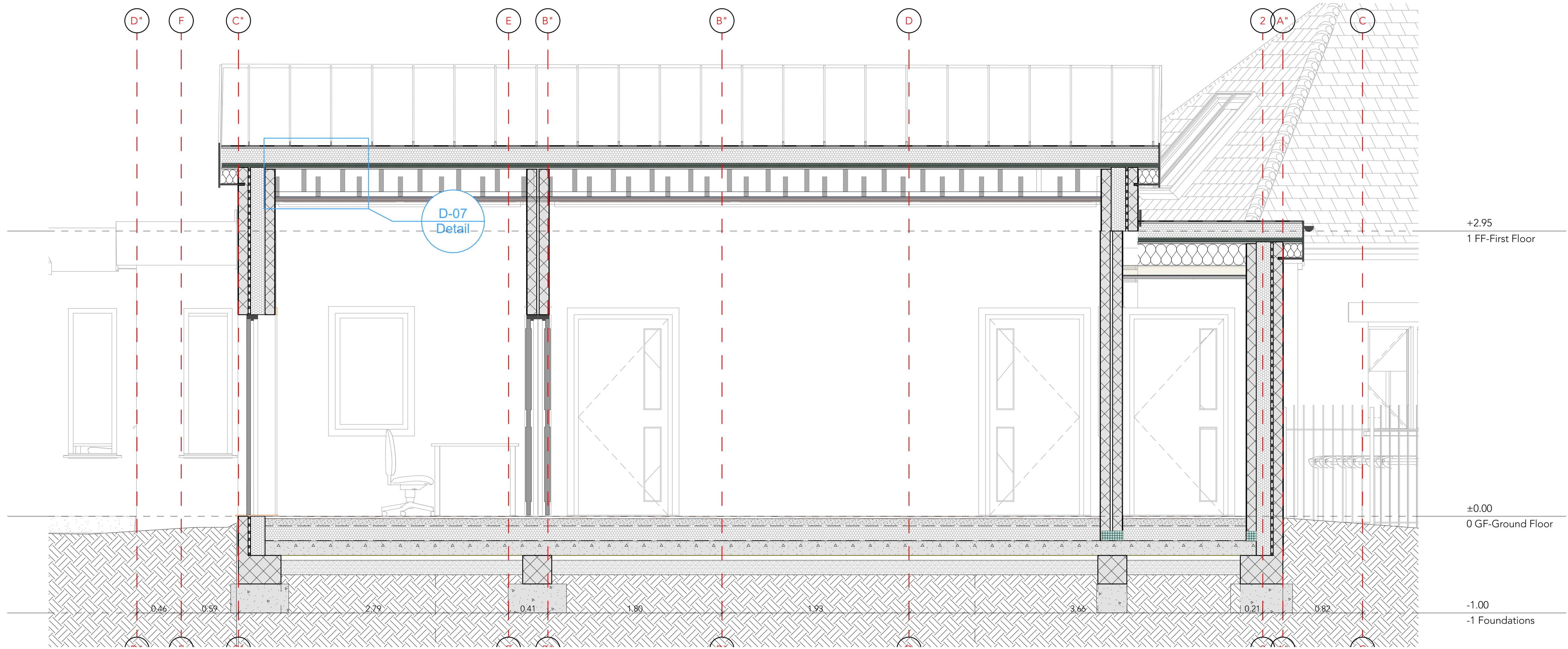
Section A
