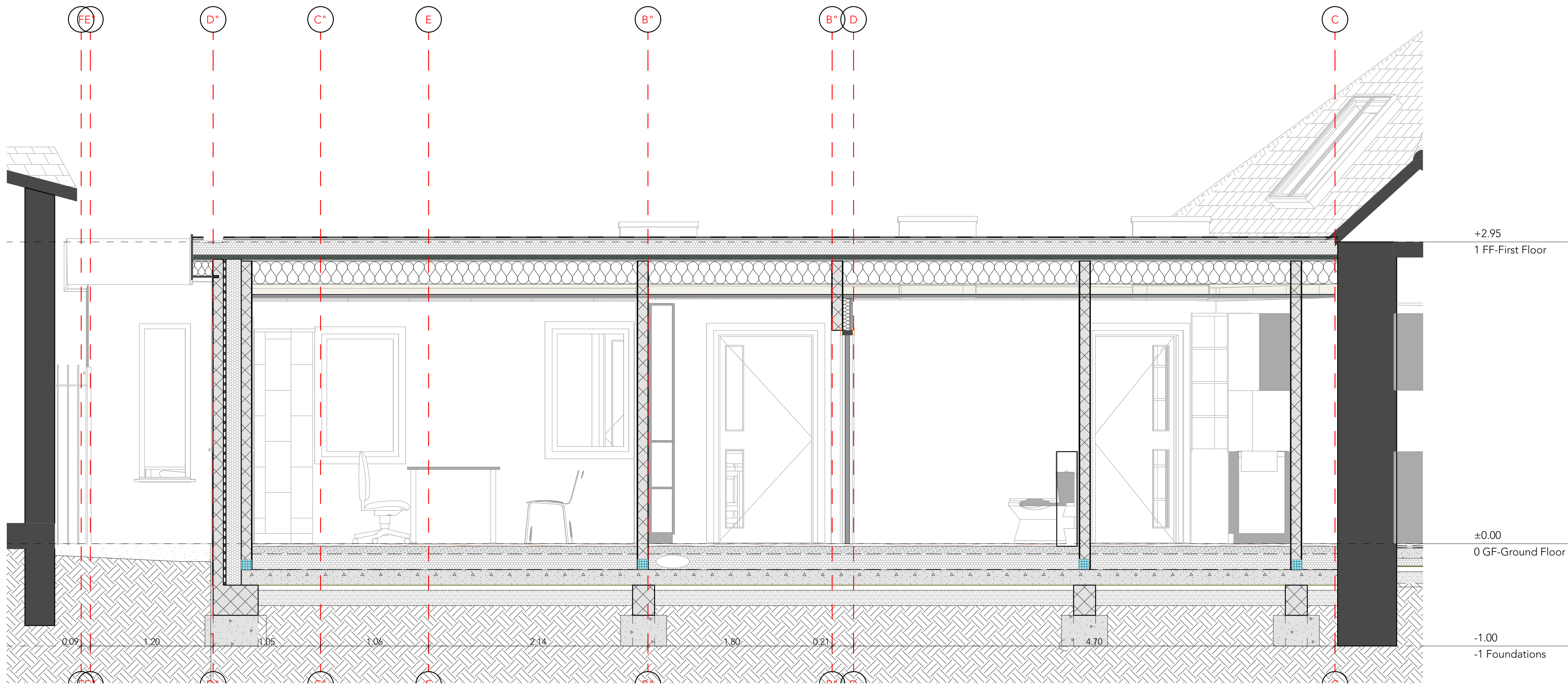
Section B
