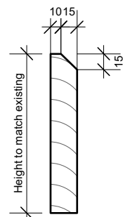
Skirting detail (to match existing) 1:5
