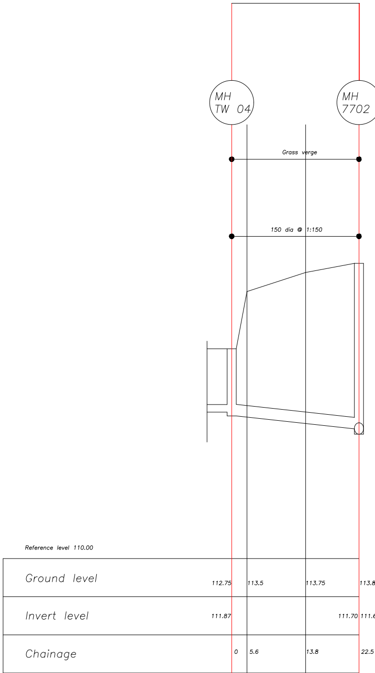
GRAVITY SEWER LONG SECTION
