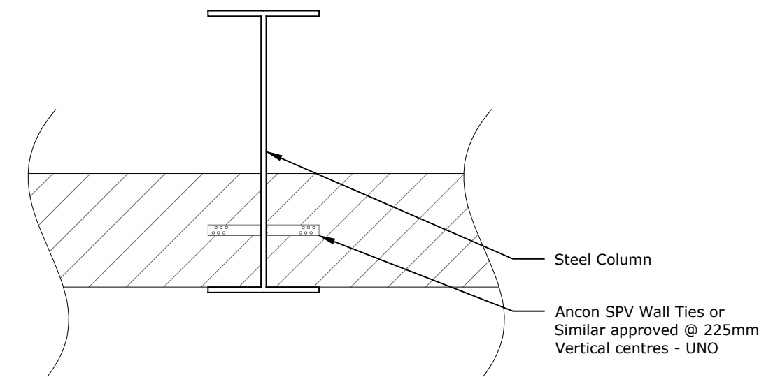
Typical vertical wall tie detail Scale 1:10
