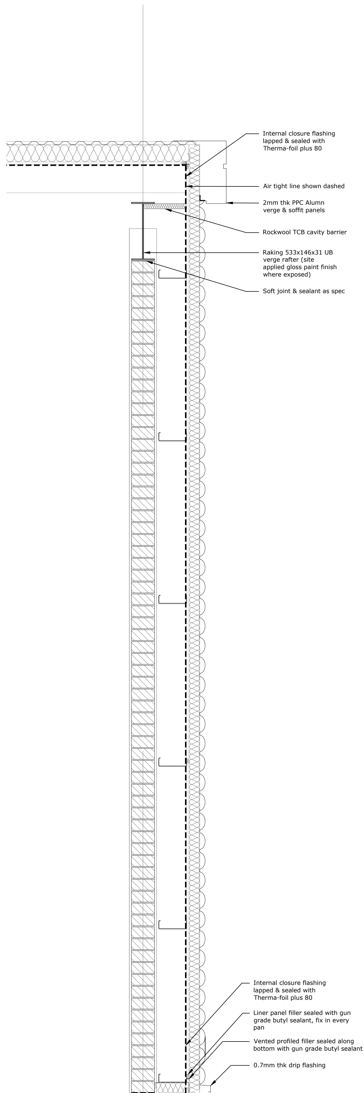
Proposed Section B Scale 1:20
