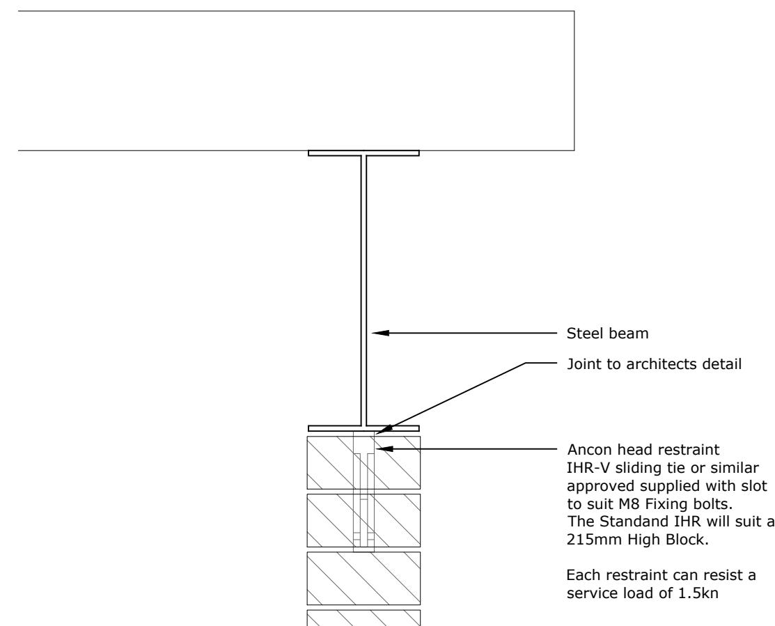
Typical wall head restraint detail Scale 1:10
