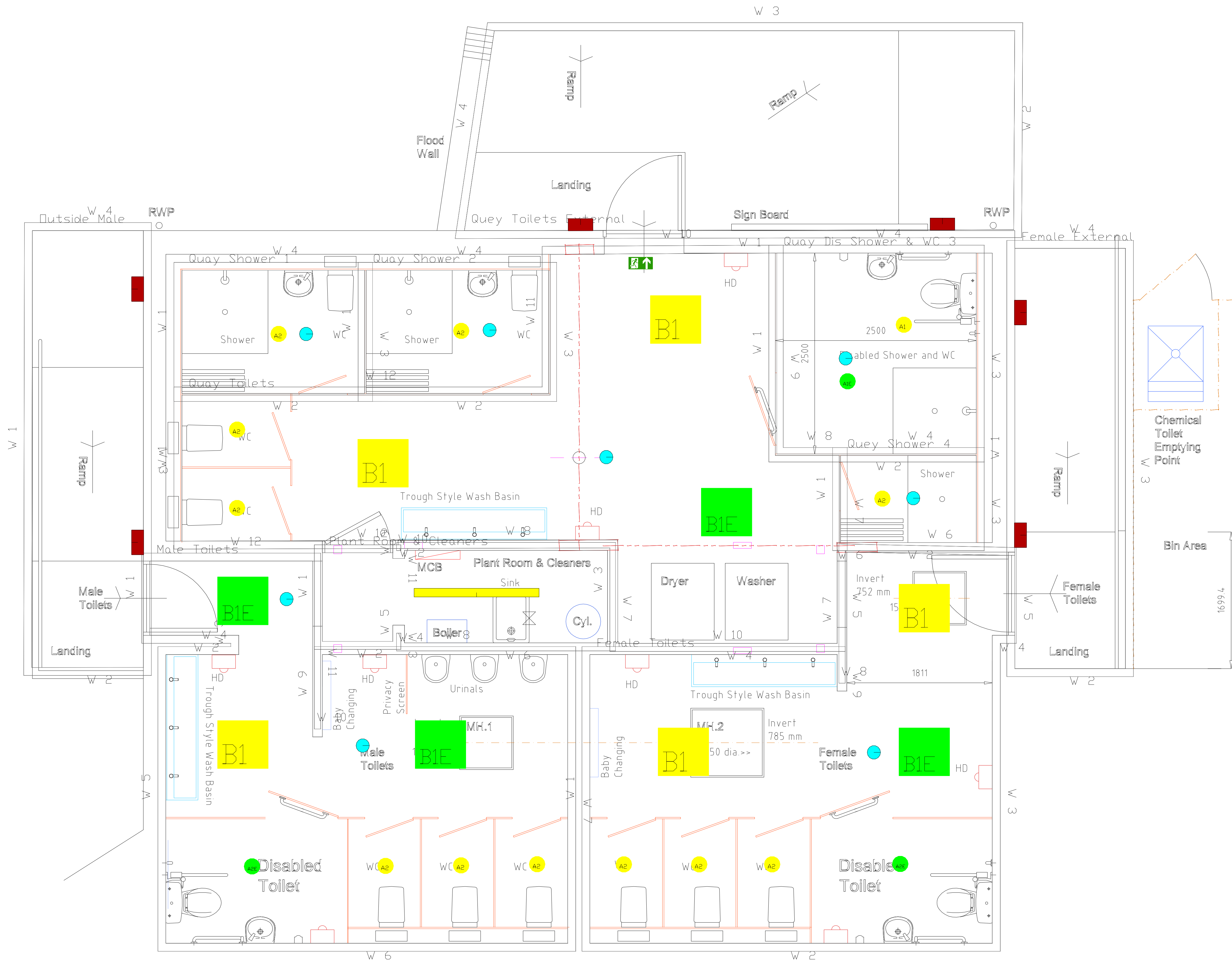
Proposed Plan Scale: 1:50
