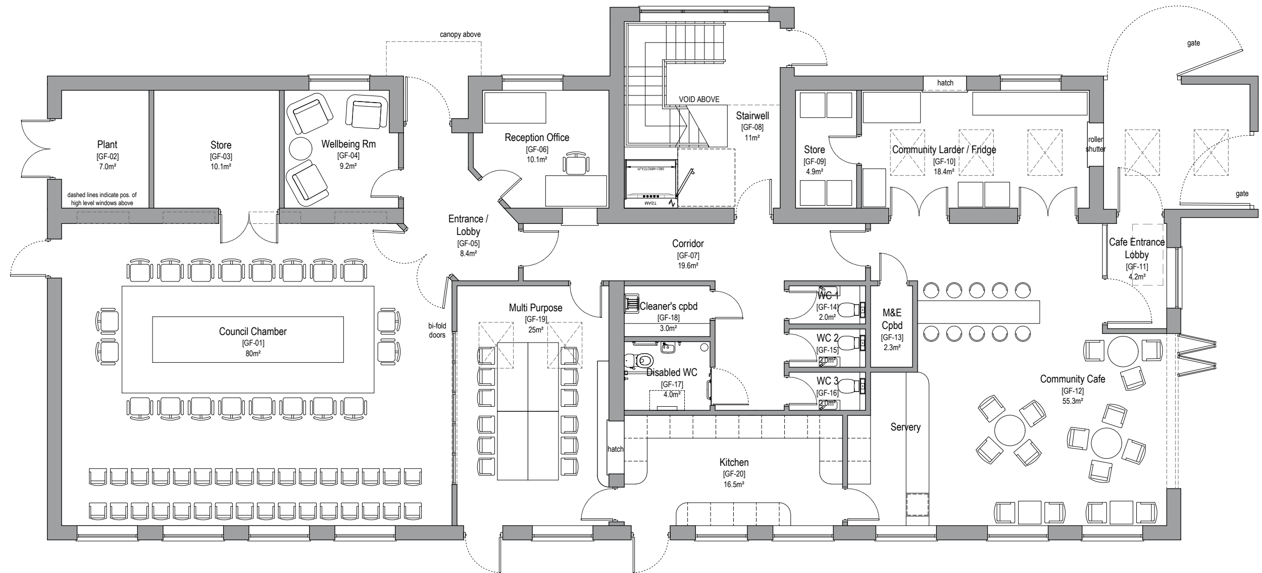
CONCEPT GROUND FLOOR PLAN
