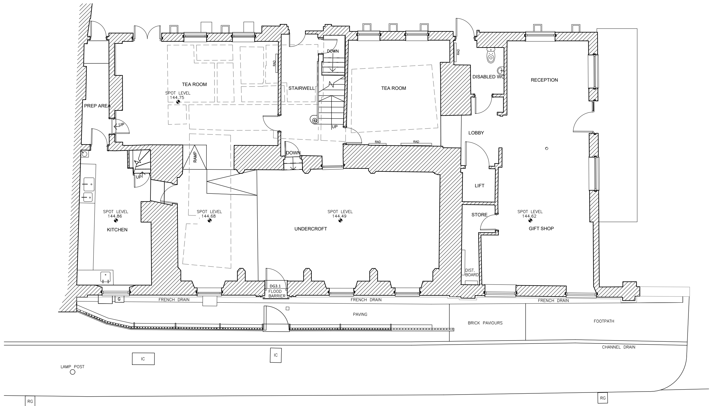
Existing Ground Floor Plan, 1:100@A3
