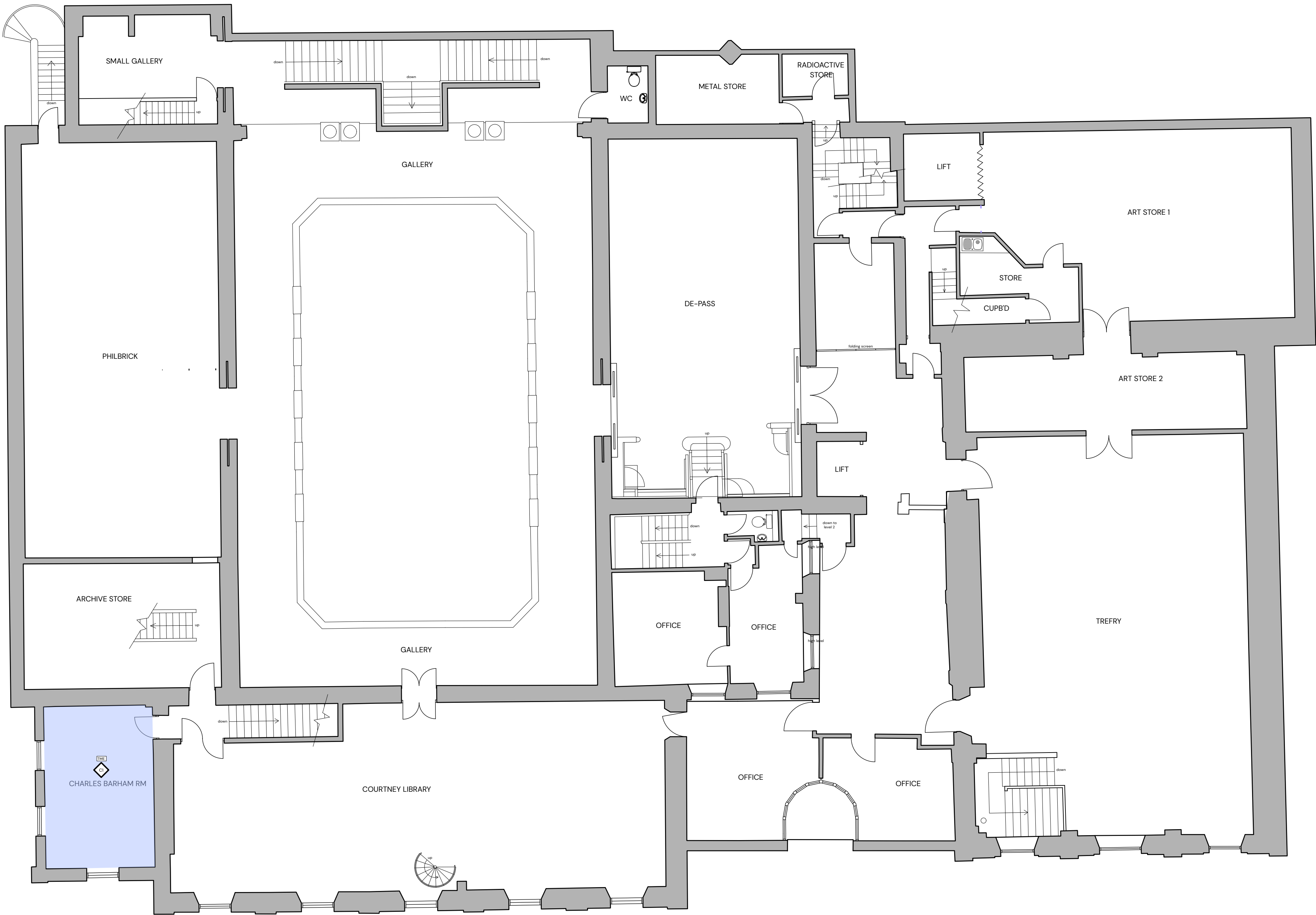
Proposed First Floor Ceiling Plan
