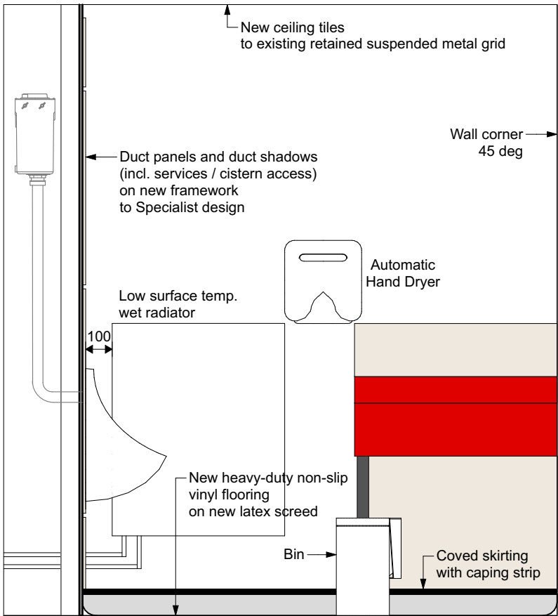
IE-02 02 Proposed Men WC 1:20
