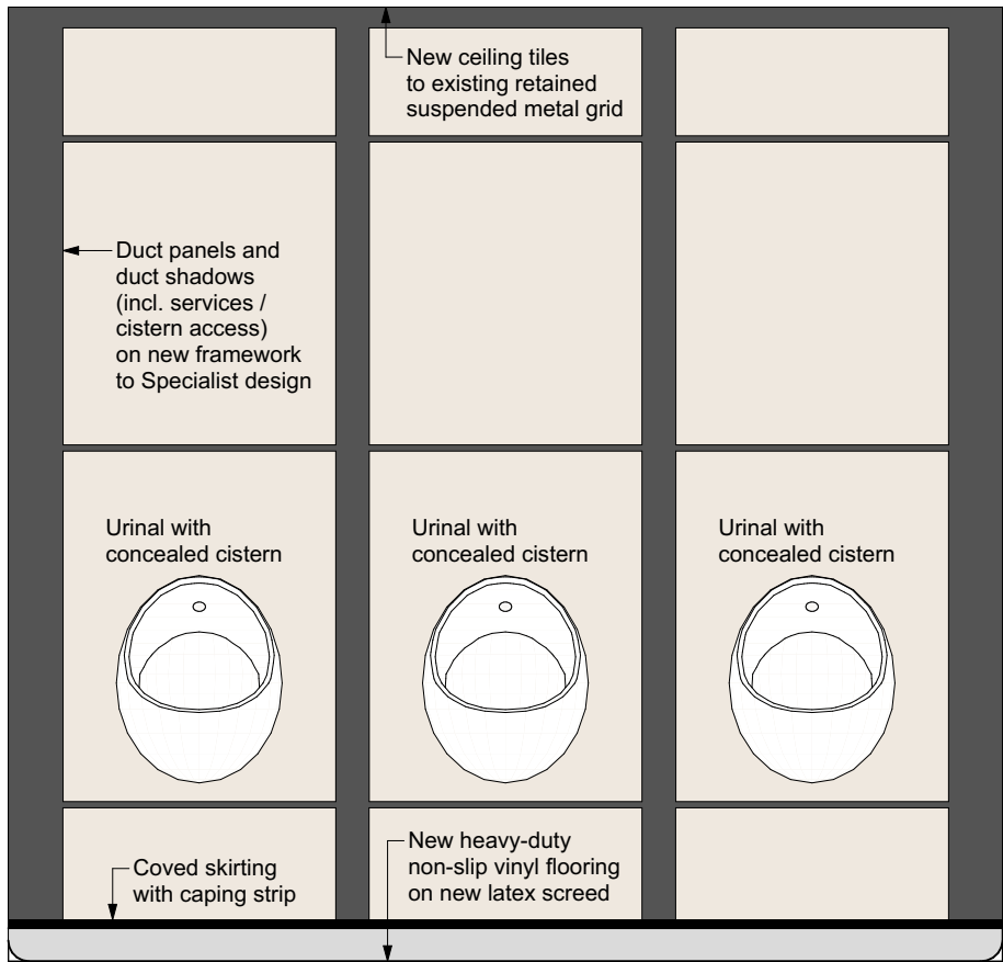
IE-02 01 Proposed Men WC 1:20
