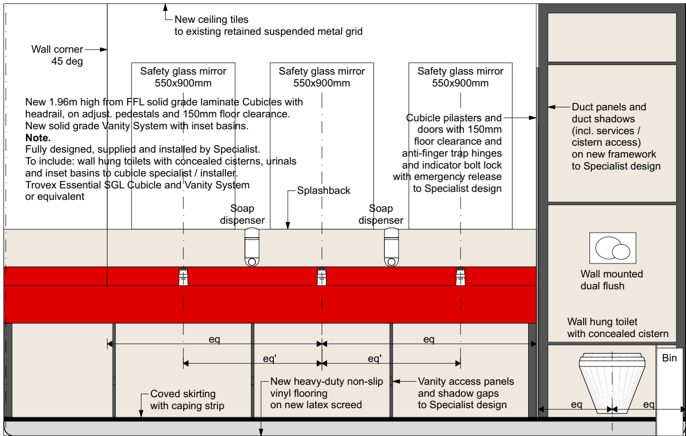
IE-02 03 Proposed Men WC 1:20
