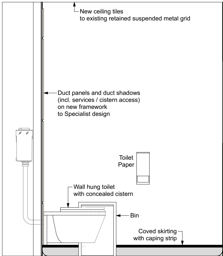
IE-02 04 Proposed Men WC 1:20
