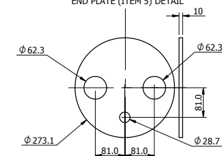
END PLATE (ITEM 5) DETAIL
