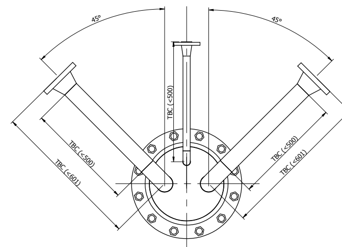
END PLATE (ITEM 5) DETAIL
