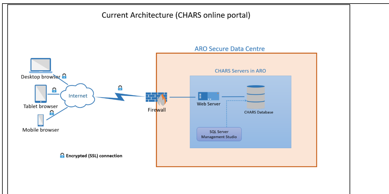
Figure 1: Current architecture of the CHARS database and online portal
