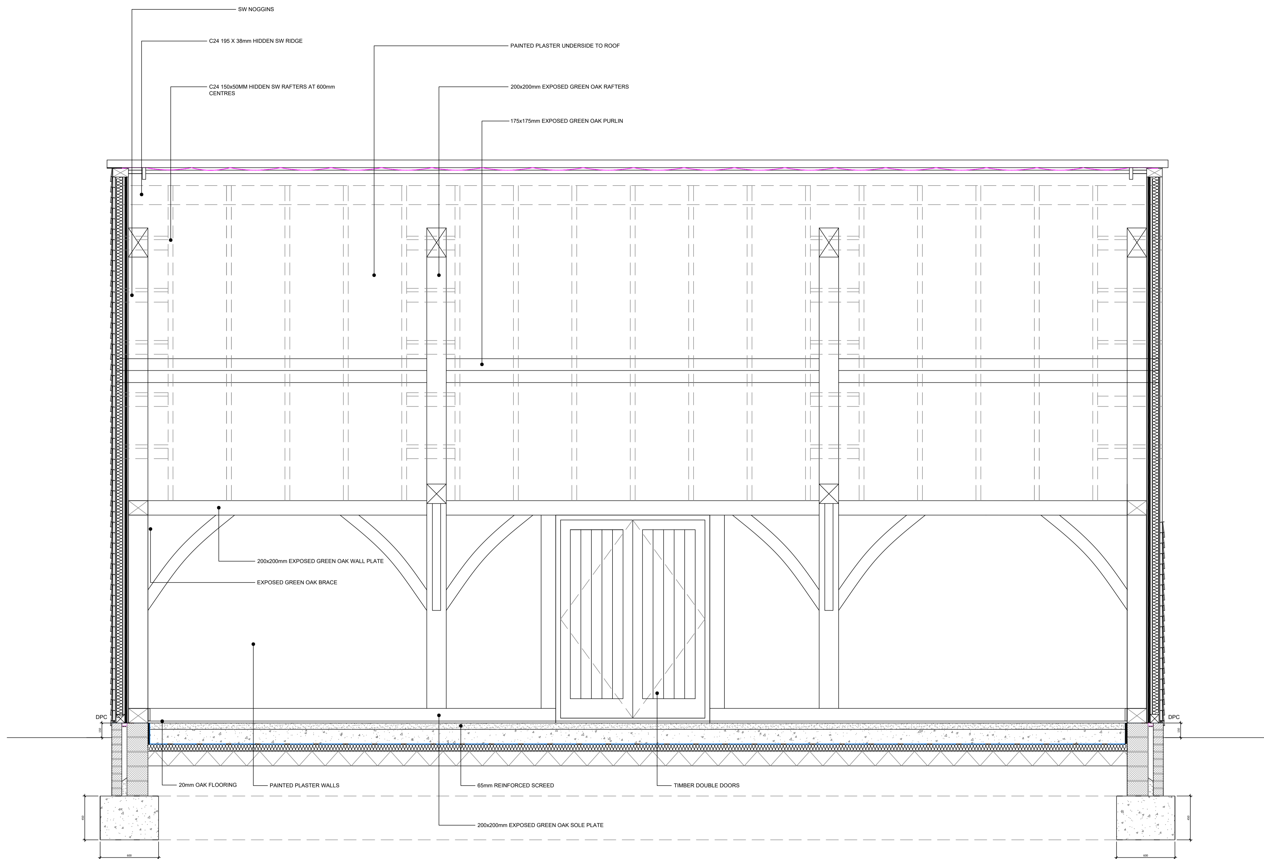
1 101 CONTEMPLATION BUILDING - SECTION A-A Scale 1:20 @ A1
