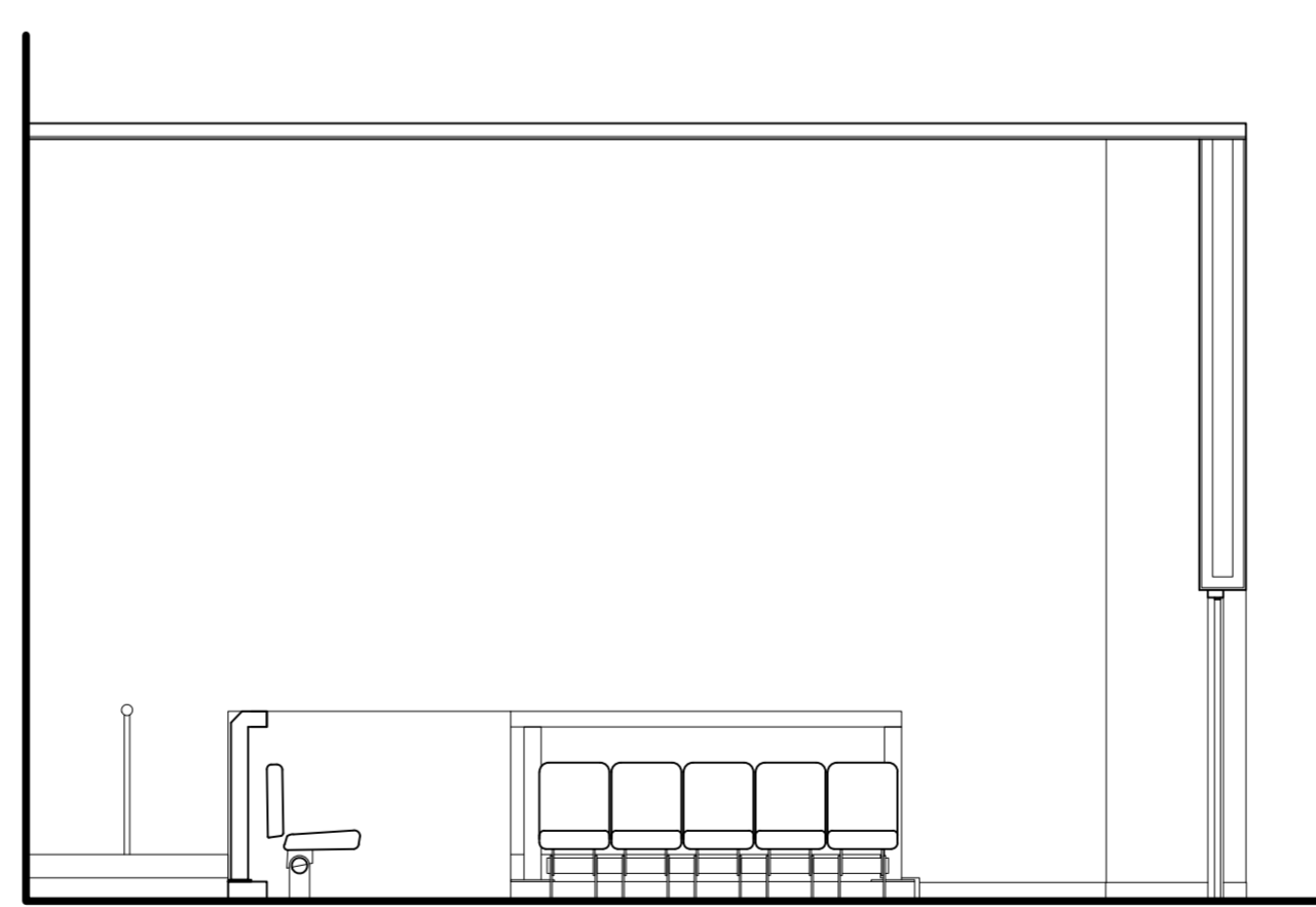
4 AREA 5.5 IMMERSIVE THEATRE ELEVATIONS Scale 1:50
