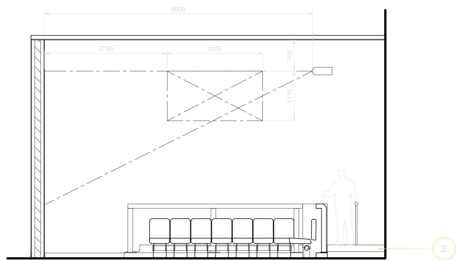
3 AREA 5.5 IMMERSIVE THEATRE ELEVATIONS Scale 1:50
