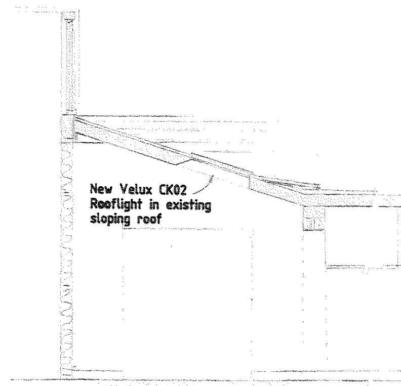
SECTION C-C
