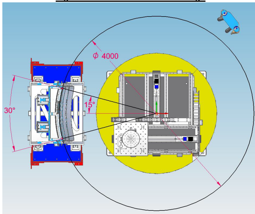
Figure 4 - Detector horizontal coverage
