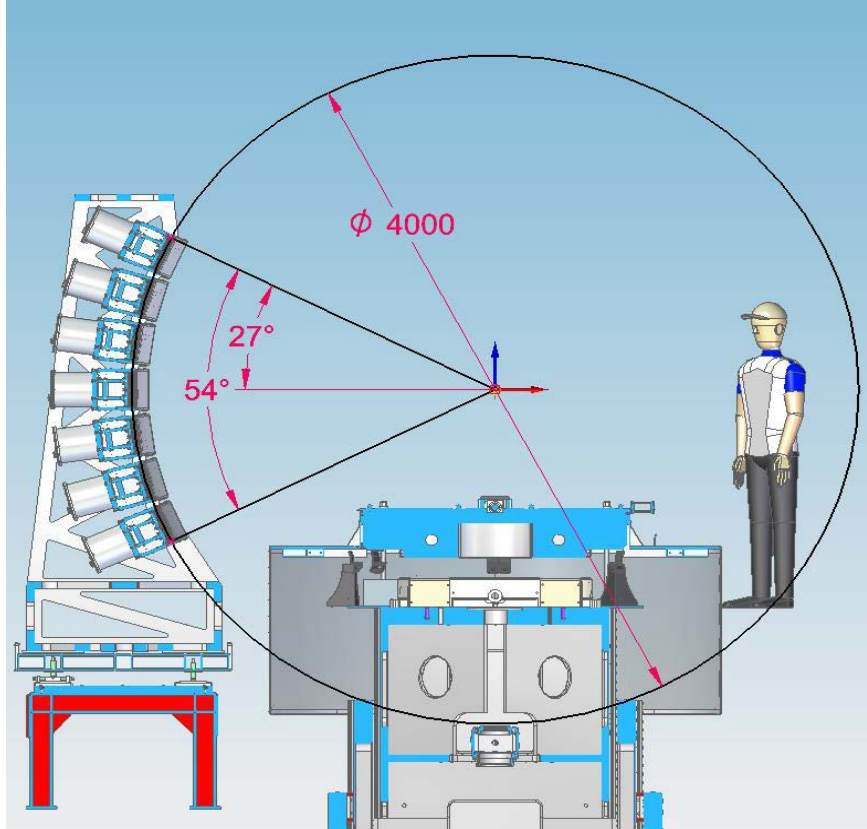
Figure 3 - Detector vertical coverage
