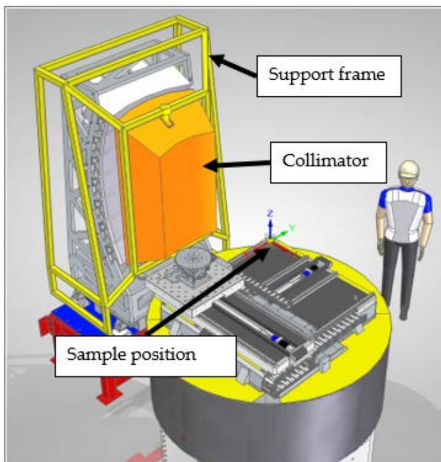
Figure 2 – Support frame example
