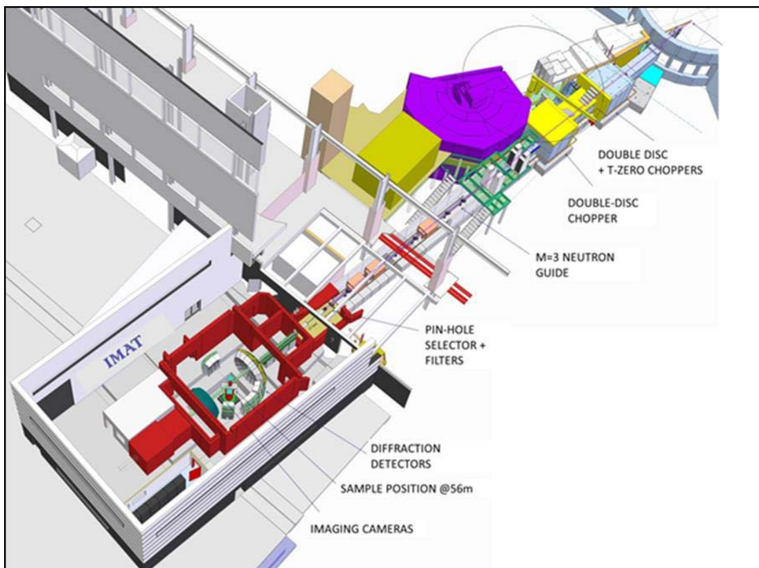
Figure 1 - IMAT layout
