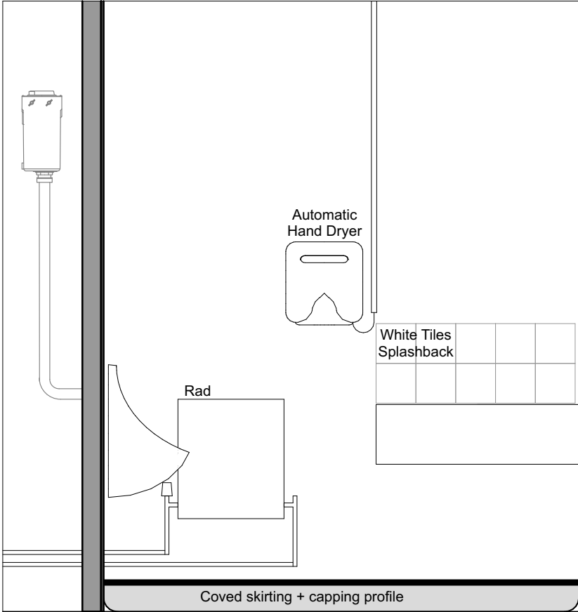
IE-02 02 Existing Men WC 1:20
