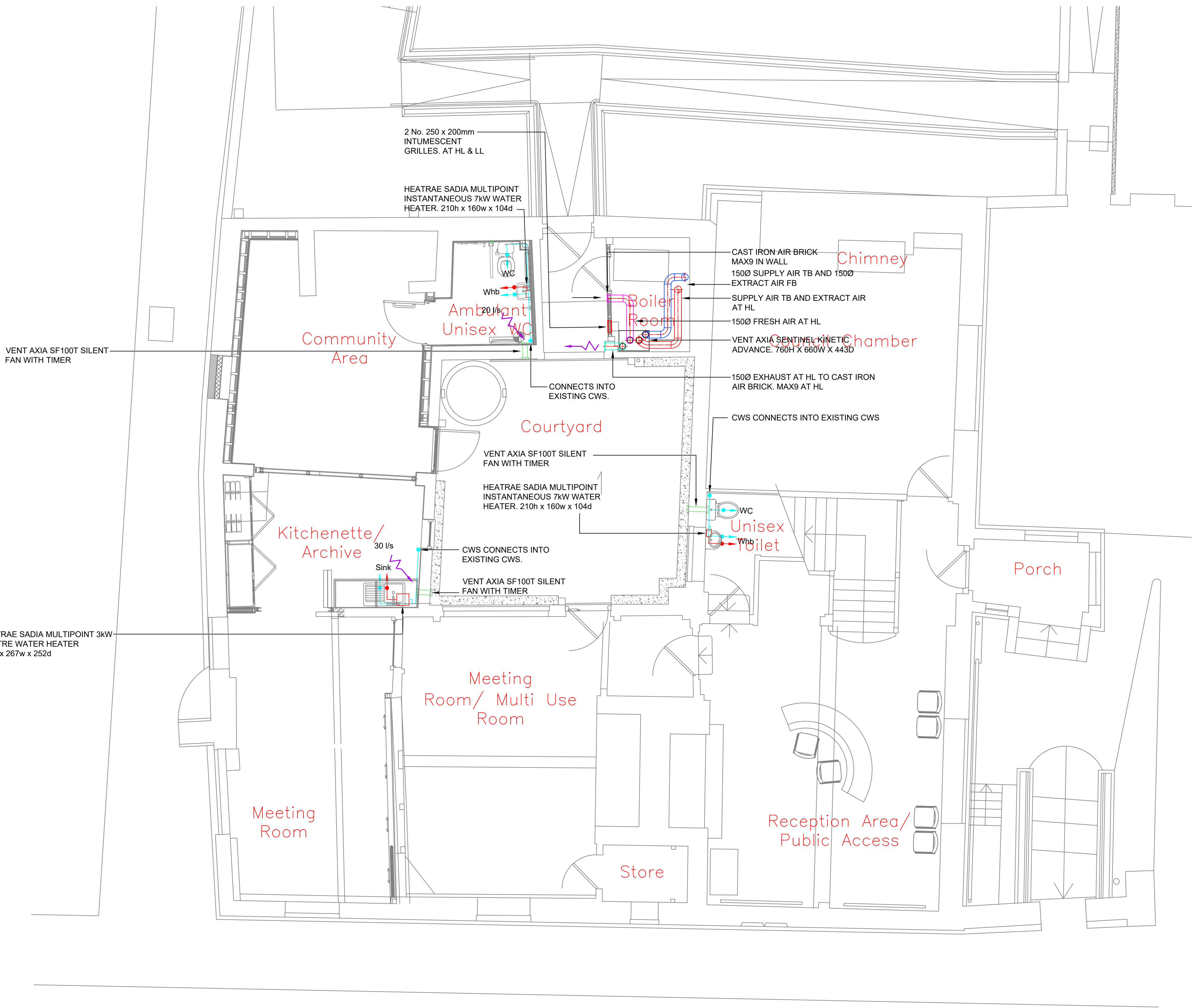
HEATRAE SADIA MULTIPOINT INSTANTANEOUS 7kW WATER HEATER Not to scale
