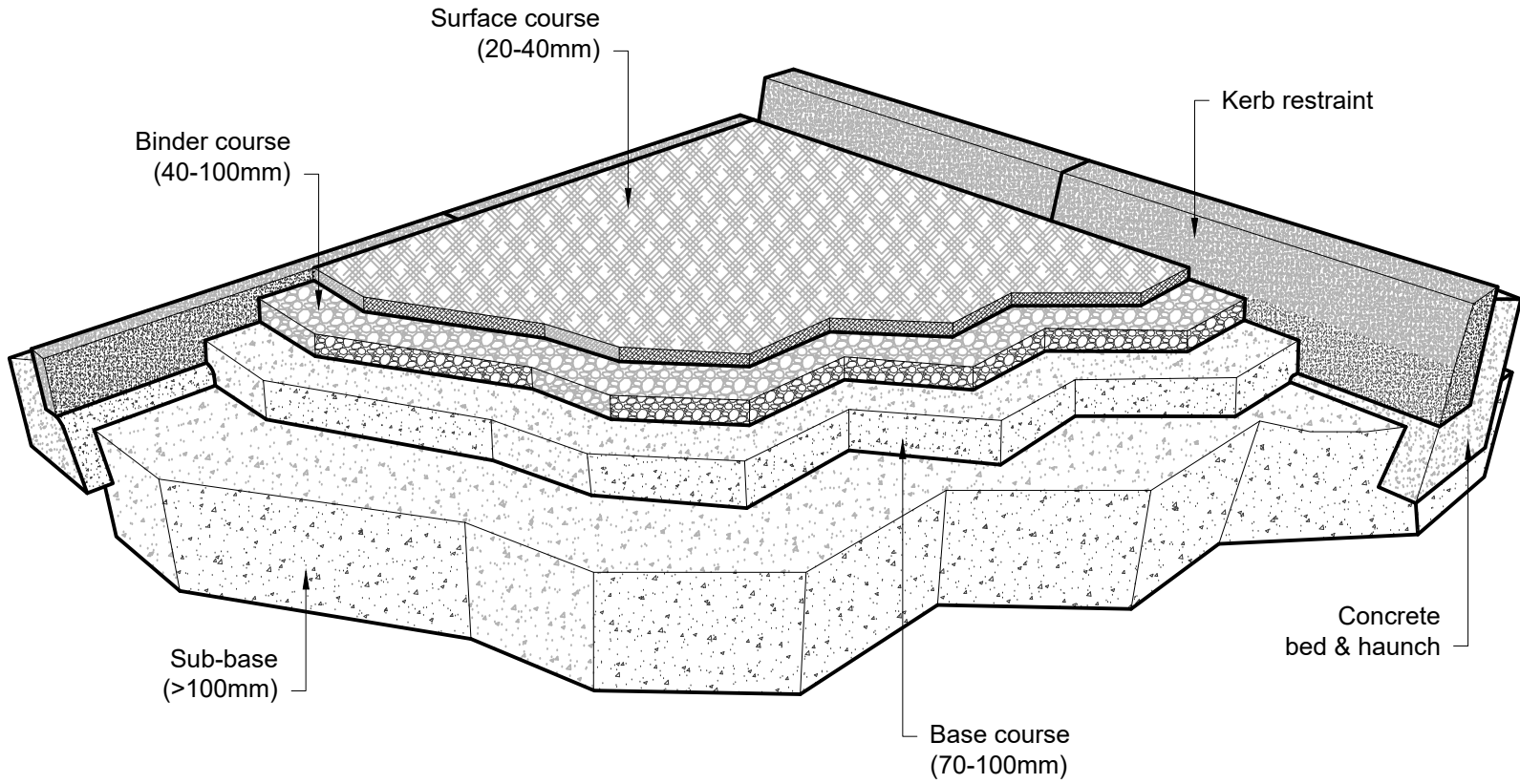
Typical Detail of Tarmac Installation
