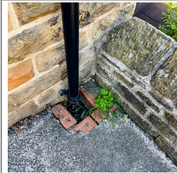
Roof: South side. Rainwater gully does not go anyway and may flood the basement. This may be better filled in and the pipe wash across the tarmac
