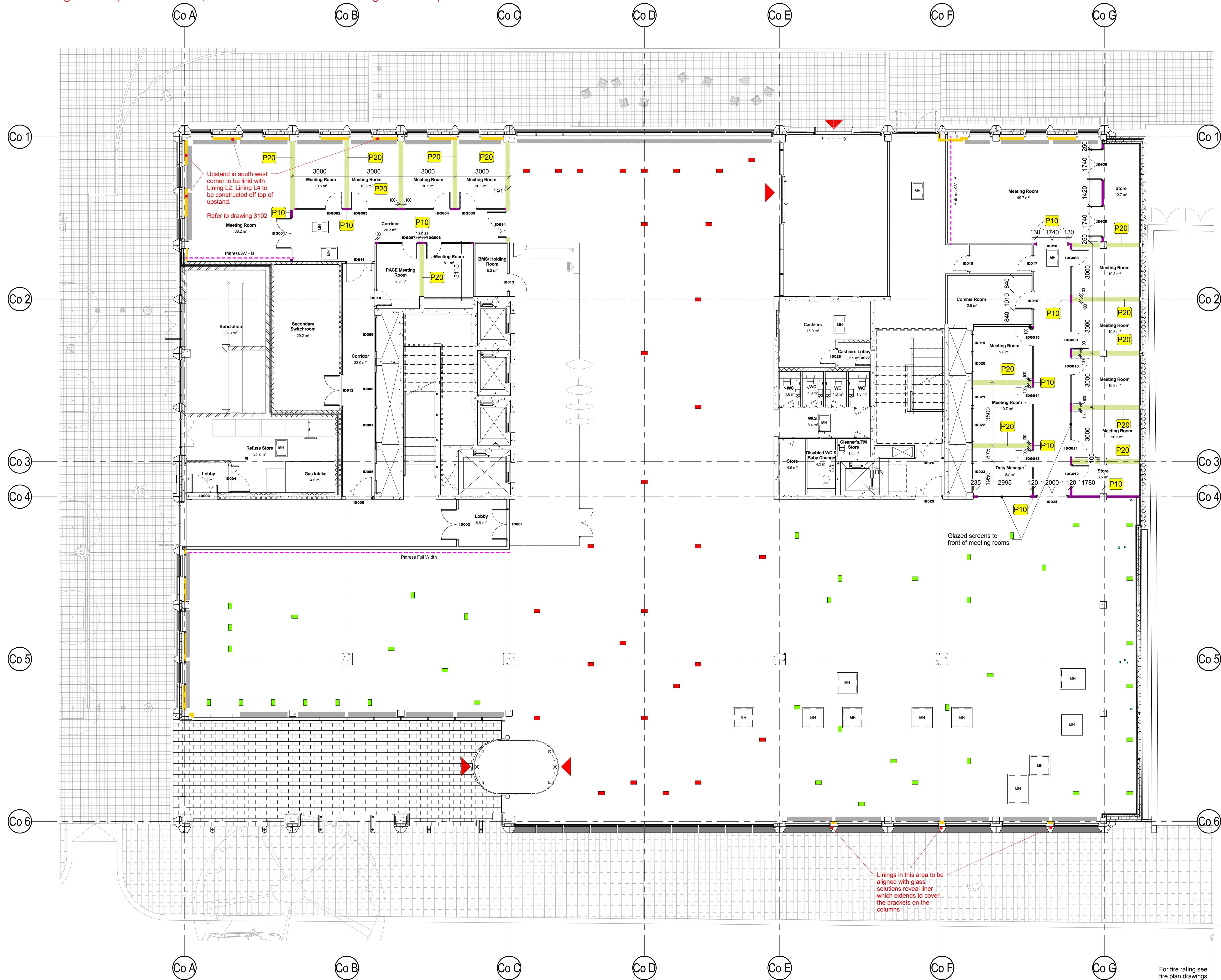
1 Ground Floor CAT B Fit Out Plan 1 : 100
