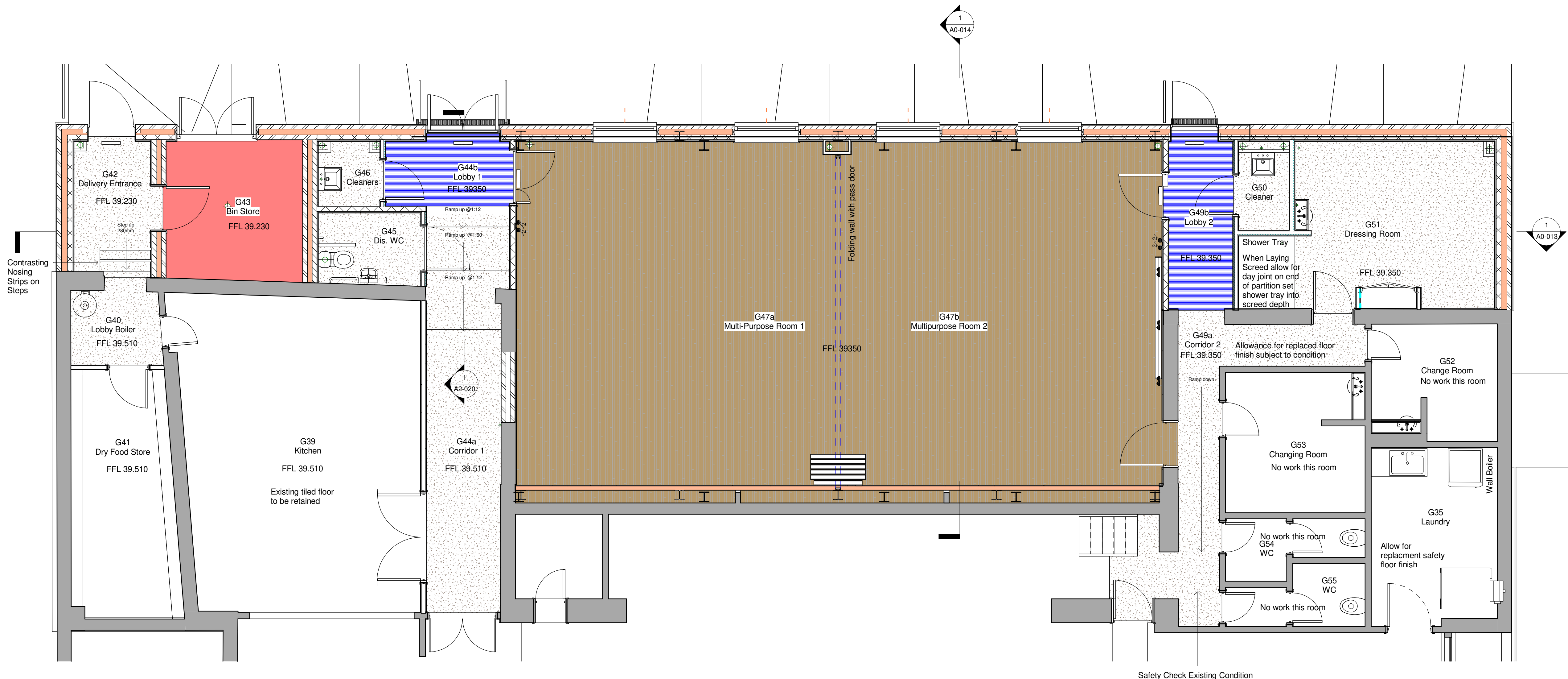
Ground Floor GA Plan 1 : 50
