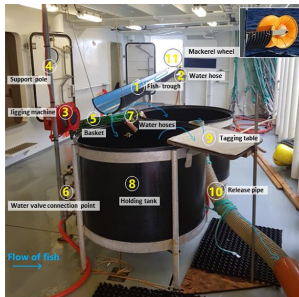
Figure 2 - Example of possible tagging setup
