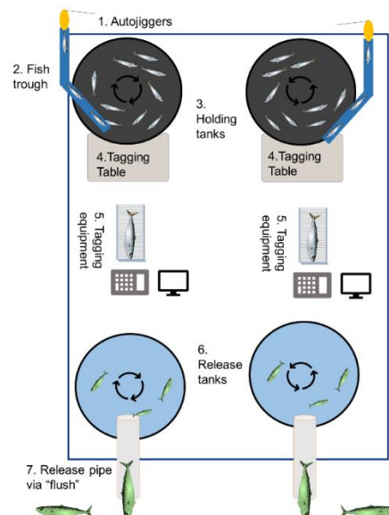
Figure 3 - Possible layout of tagging equipment on deck to be finalised during discussions with selected vessel and crew
