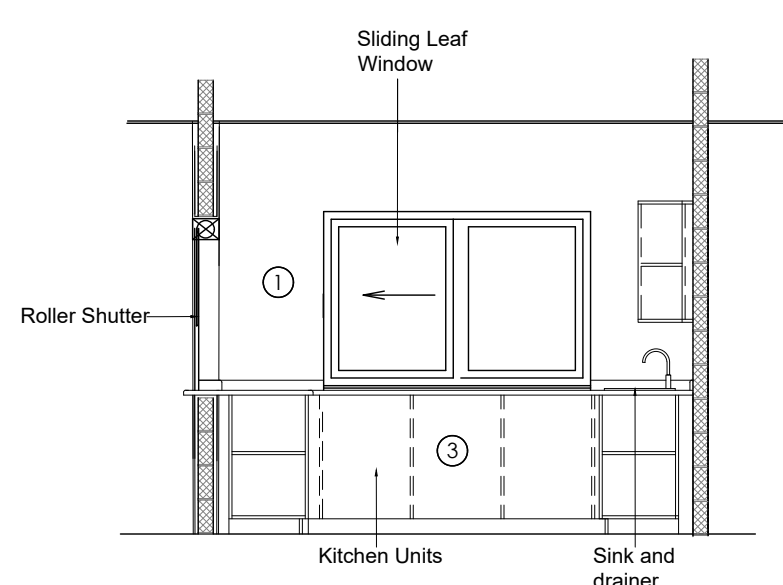
Elevation C
