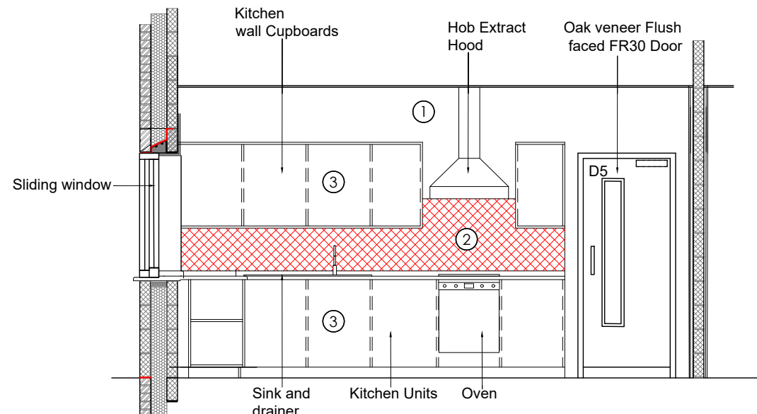
Elevation D
